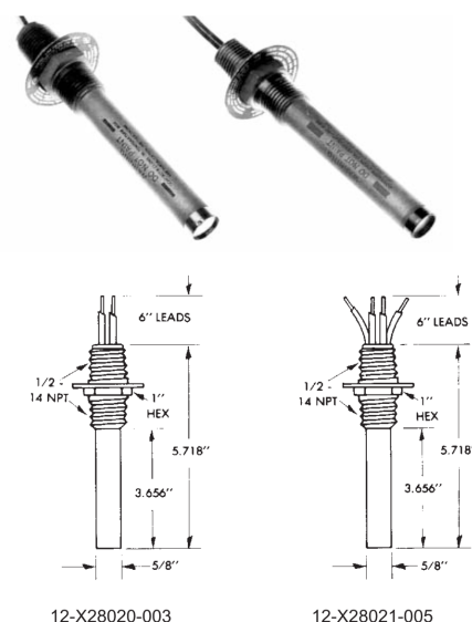
Figure 5. Coupling Head
