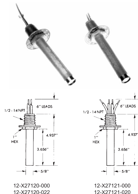
Figure 4. Hexagonal Head
